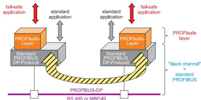
Rys. 1. Tryb pracy failsafe z profilem PROFIsafe
